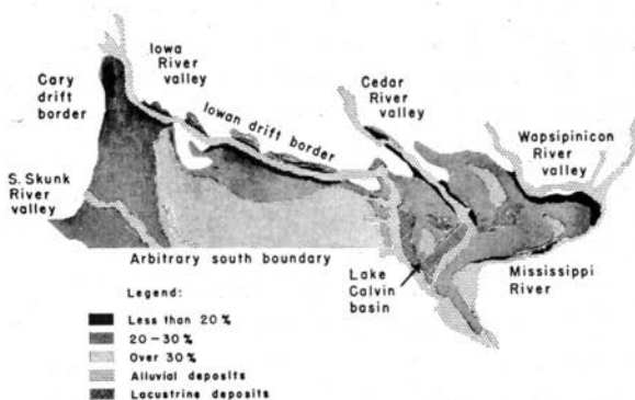
Fig. 5 Approximate areal variation in the clay content ( <0.005\text{mm} ) of the C horizon Wisconsin loess in east-central Iowa.
