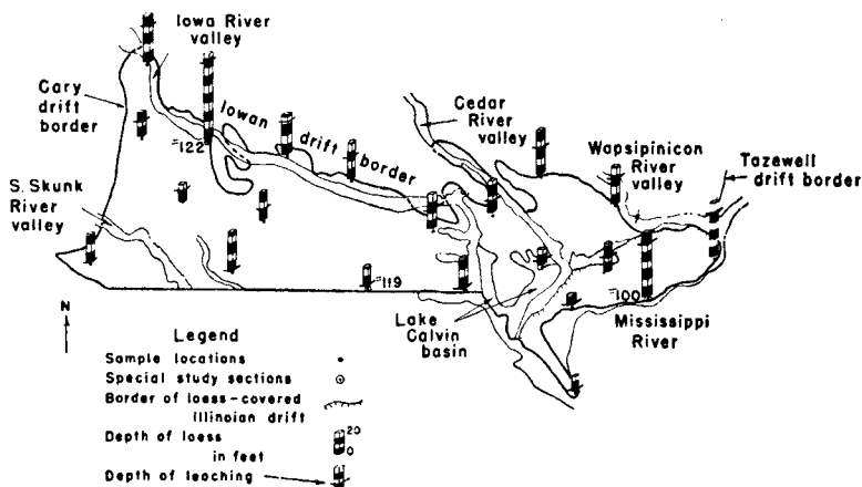
Fig. 2 Depth of Wisconsin loess at sampling locations in east-central Iowa
