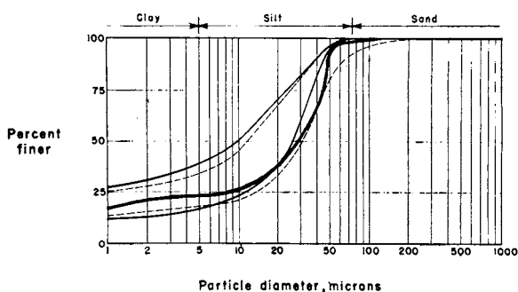
Fig. 13. The heavy line indicates particle sizes of dust which settled in Garden City, Kansas. Other particle size curves are for Wisconsin-age loess in Iowa. The solid lines are for typical samples from southwestern Iowa, the dashed lines for typical samples from east-central Iowa.
