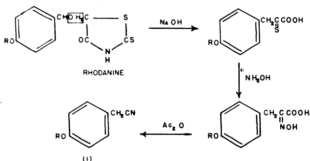
Chart I. Synthesis of phenylacetonitriles.
