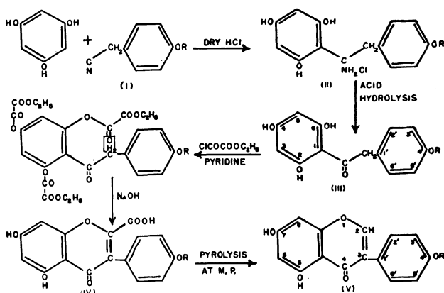
Chart II. Synthesis of isoflavones.
