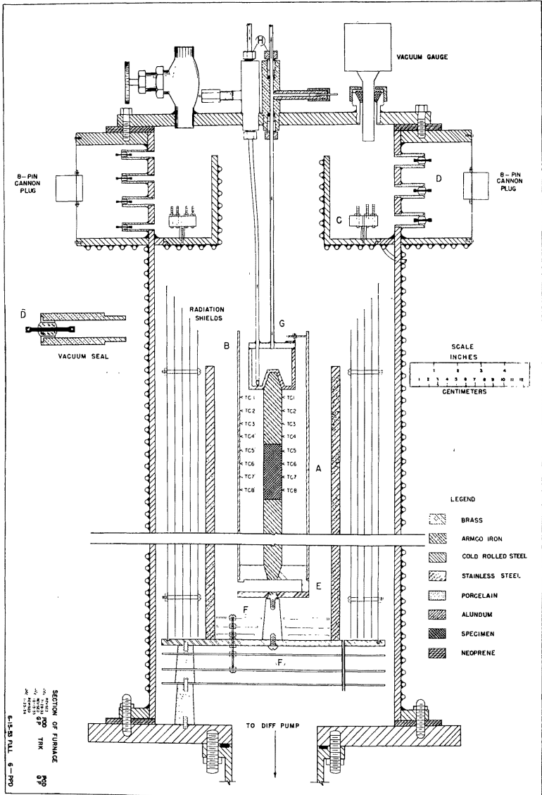
Figure 1. Vacuum Furnace for Thermal Conductivity Measurements.
