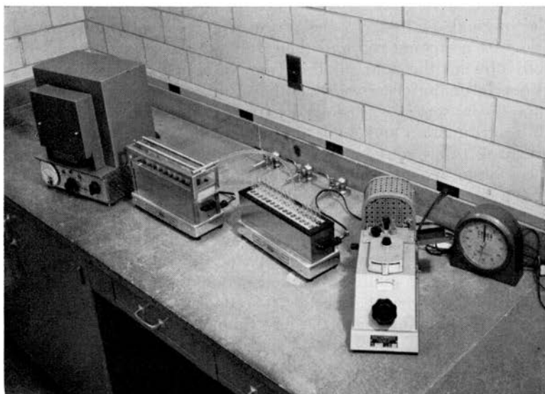
Figure 3. Instruments used for PBI determination. From left to right are the Thermolyne muffle furnace, the dri-bath with aeration rack in place, the special dri-bath containing 30 holes for Klett colorimeter tubes, the Klett colorimeter and timer.
