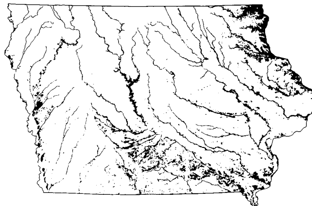
Fig. 2 Present forest in Iowa redrawn from remote-sensing, satellite photography gathered data as presented in Land-Use in Iowa, Miscellaneous Map Series 5 , Iowa Geological Survey, 1976.
