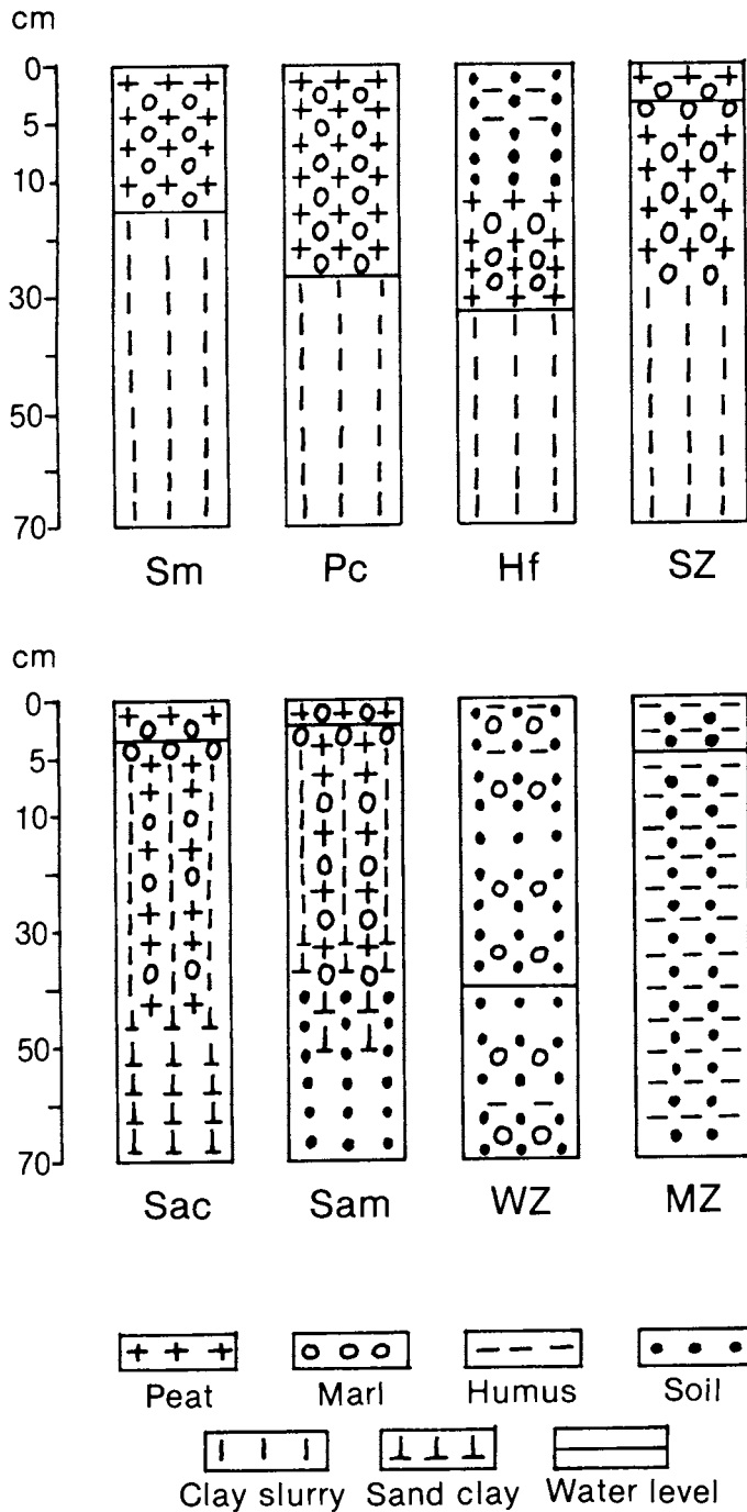
Fig. 2. Substrate profiles for vegetation zones at Silver Lake fen complex.
