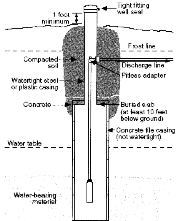
Fig. 2. Typical construction of buried slab wells (Iowa State University 1993b).
