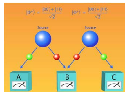
Figure 1. Simplified depiction of experiments to show that complex numbers are necessary in standard quantum mechanics.
